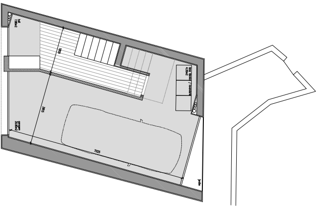
01 PIANO (m 2 )
