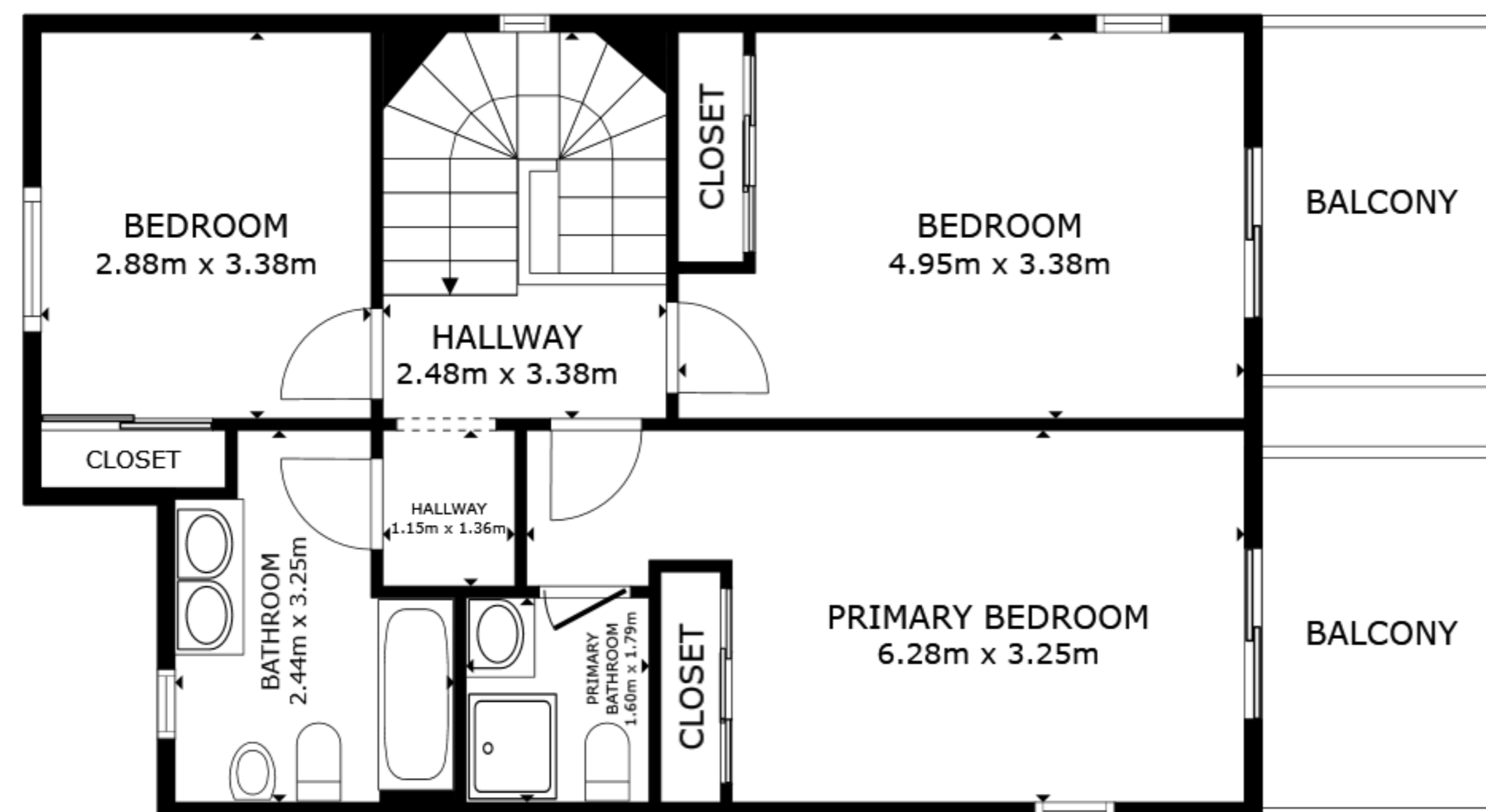
FLOOR 2
