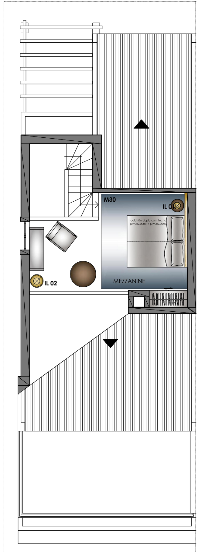
PLANTA MEZZANINE
